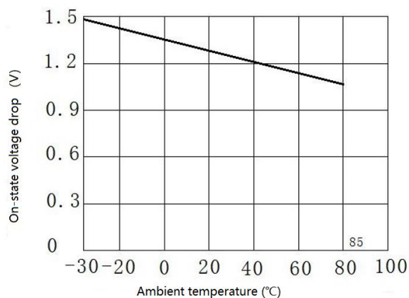
● On-state voltage drop vs Ambient Temperature
