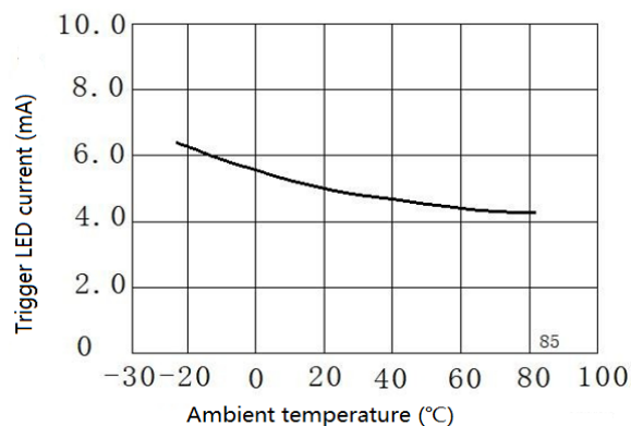
● Trigger LED current vs Ambient Temperature
