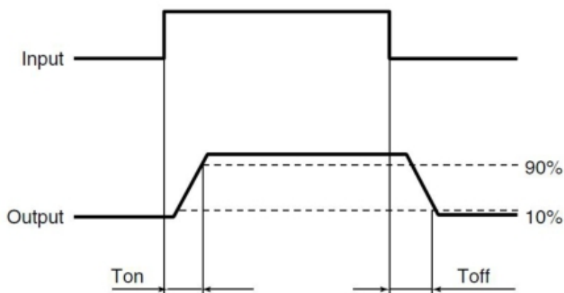
● Turn-on and turn-off time
